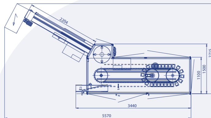
Overall dimensions (mm): 5570 x 2715 x H1880
