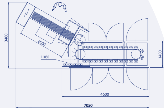
Overall dimensions (mm): 7050 x 3480 x H2300
