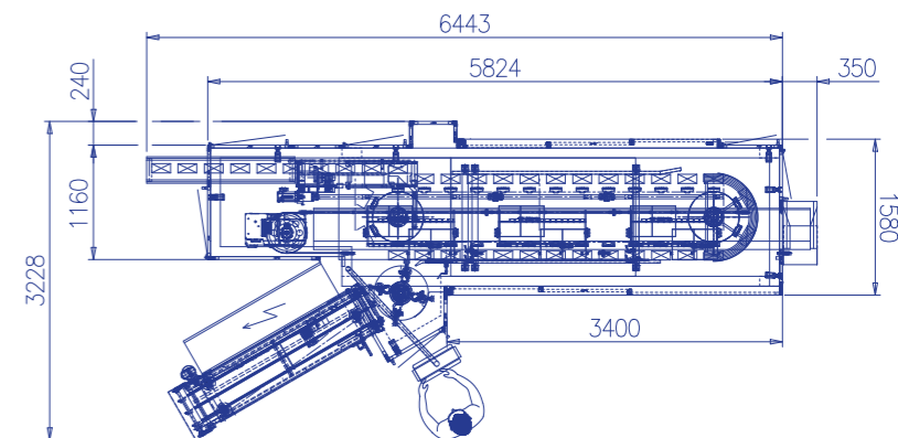
Overall dimensions (mm): 6440 x 3200 x H2300
