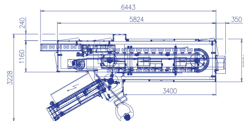
Overall dimensions (mm): 6440 x 3200 x H2300
