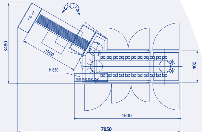
Overall dimensions (mm): 7050 x 3480 x H2300
